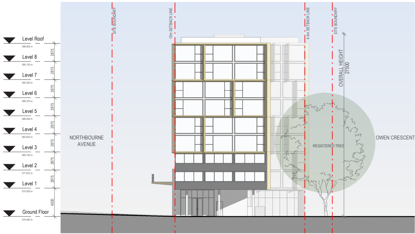
NORTH ELEVATION
