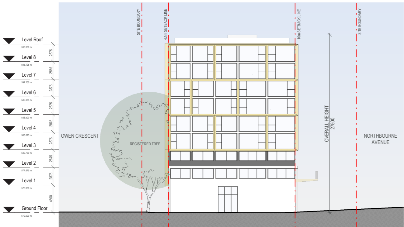
SOUTH ELEVATION
